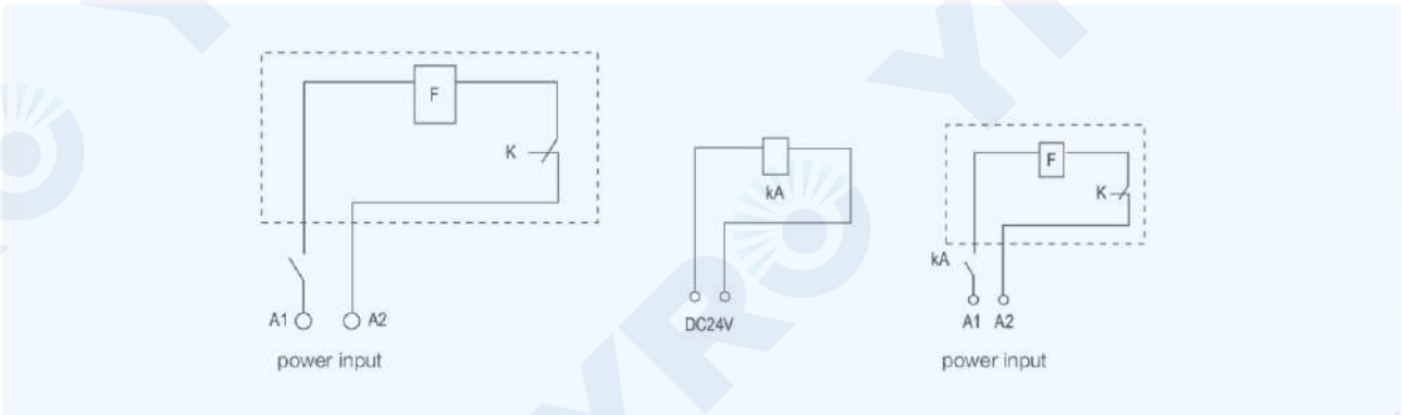
Wiring diagram of excitation tripping
