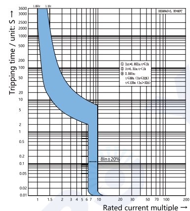
C Curve 8-10In±20% Applicable rated current ≤63A
