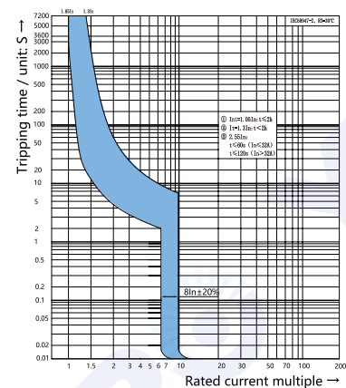
C Curve 8In ± 20% Applicable rated current 80A-125A
