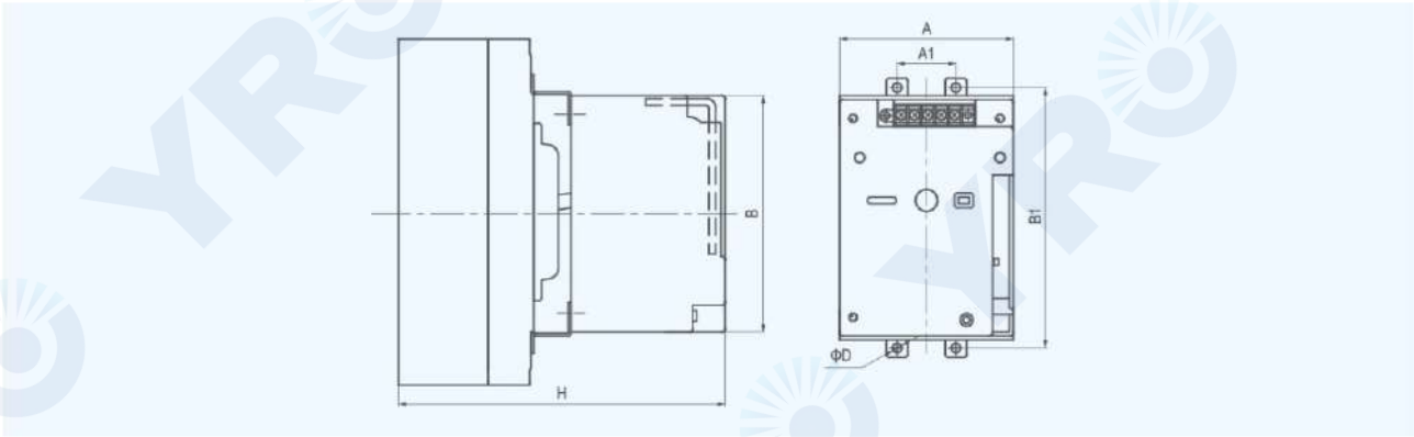
CD2 Outline and installation dimensions schematic diagram
