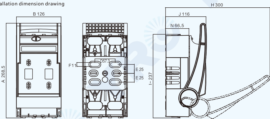
YROPV-250 Installation dimension drawing
