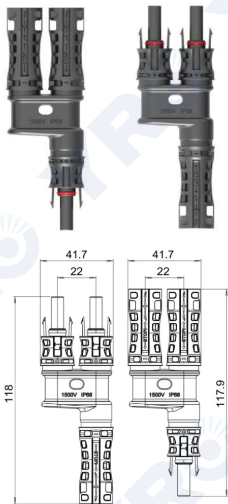
PV-LT2-A Branch Connector
