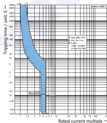
B Curve 4-6In±20% Applicable rated current ≤63A
