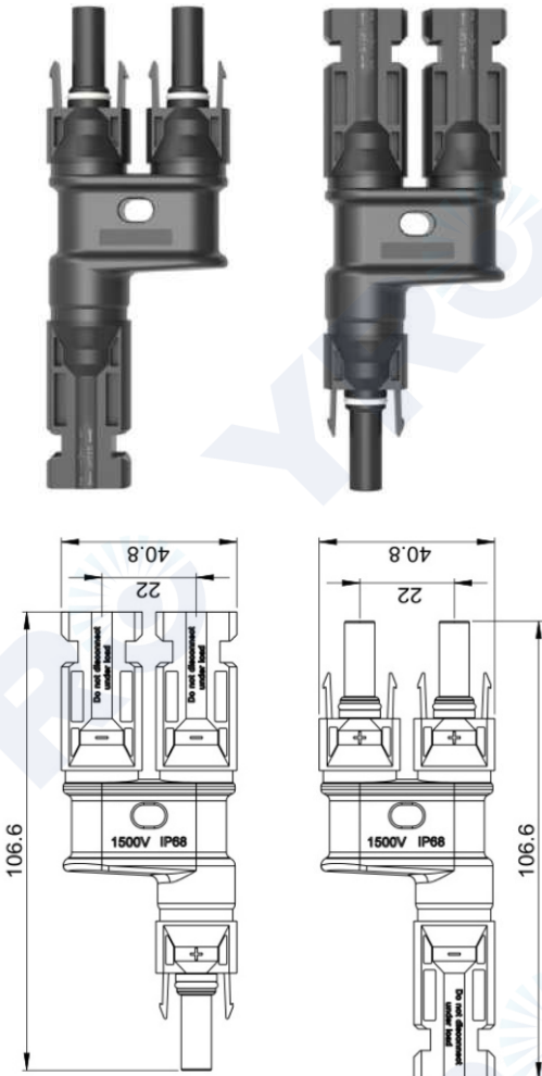
PV-LT2-B Branch Connector
