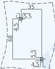
Bottom screw installation size
